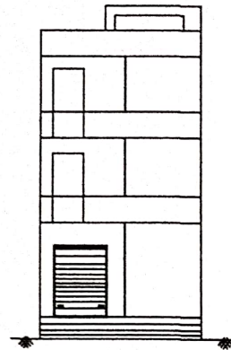
FRONT ELEVATION
