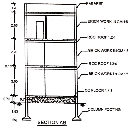
SECTION AB
