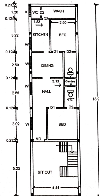
FLOOR 02
