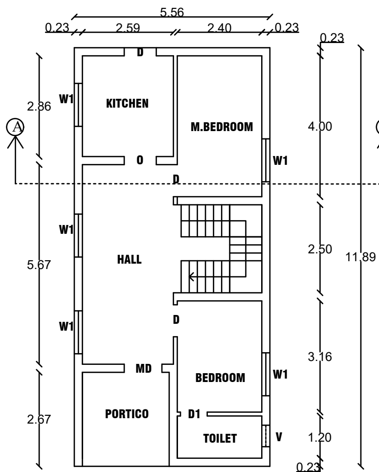
GROUND FLOOR PLAN NORTH FACING PLAN
