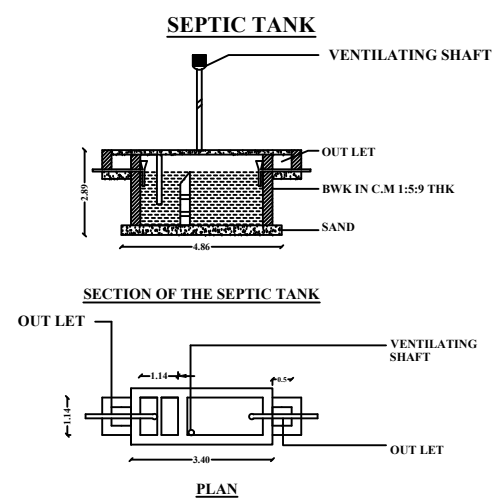
SEPTIC TANK
