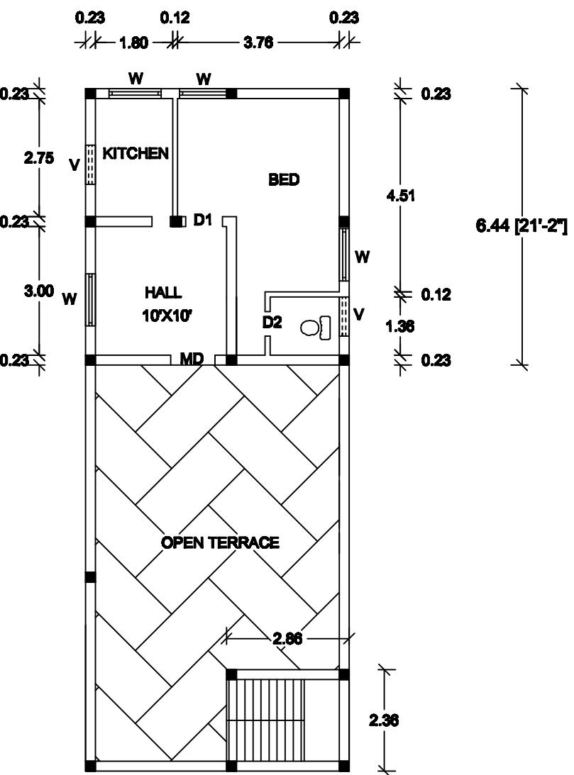
FLOOR02
