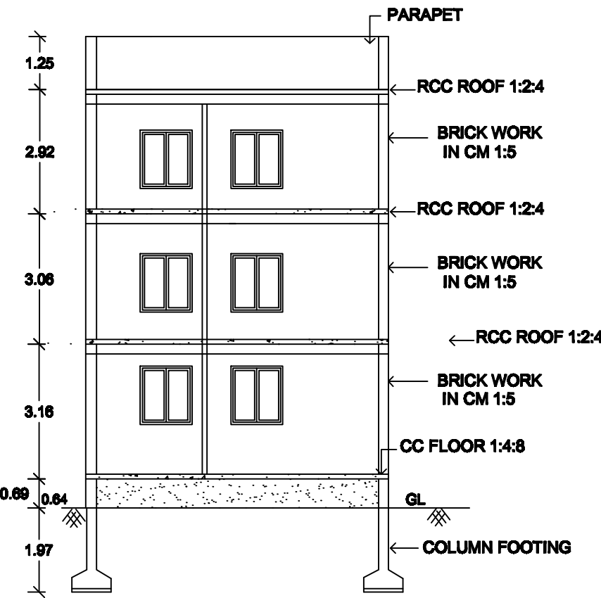
SECTION AB
