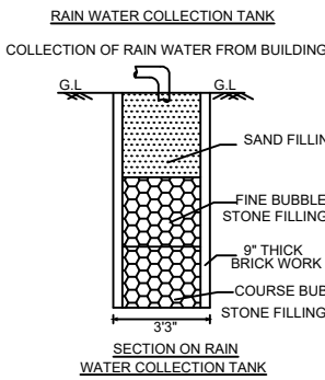
SECTION ON RAIN WATER COLLECTION TANK
