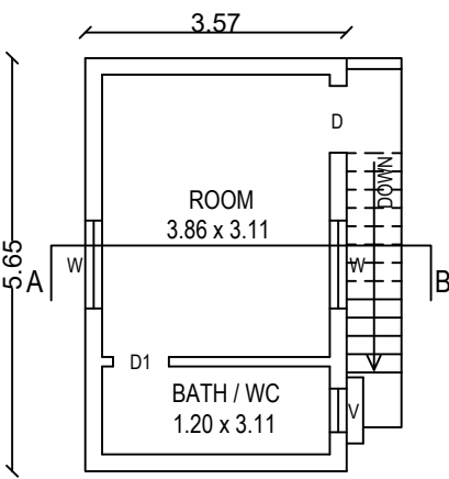
FIRST FLOOR NORTH FACING
