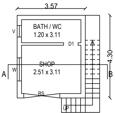
GROUND FLOOR NORTH FACING
