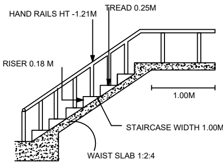
STAIRCASE DETAILS
