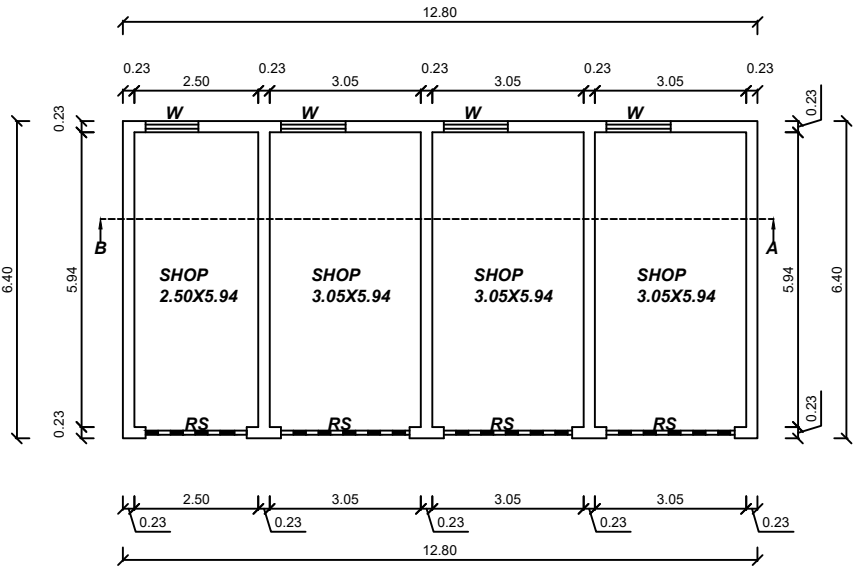
FOR PLAN
