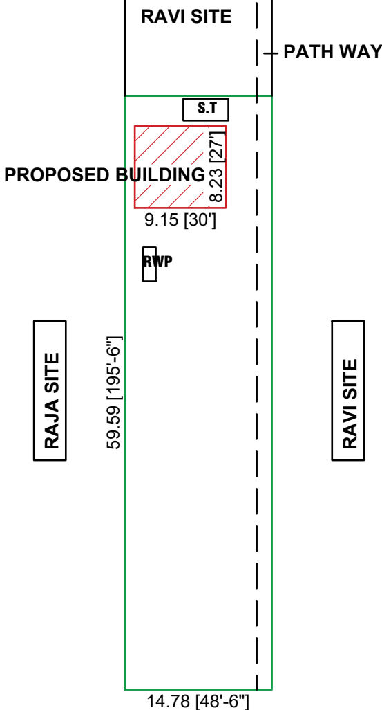
SITE PLAN SCALE 1:500
