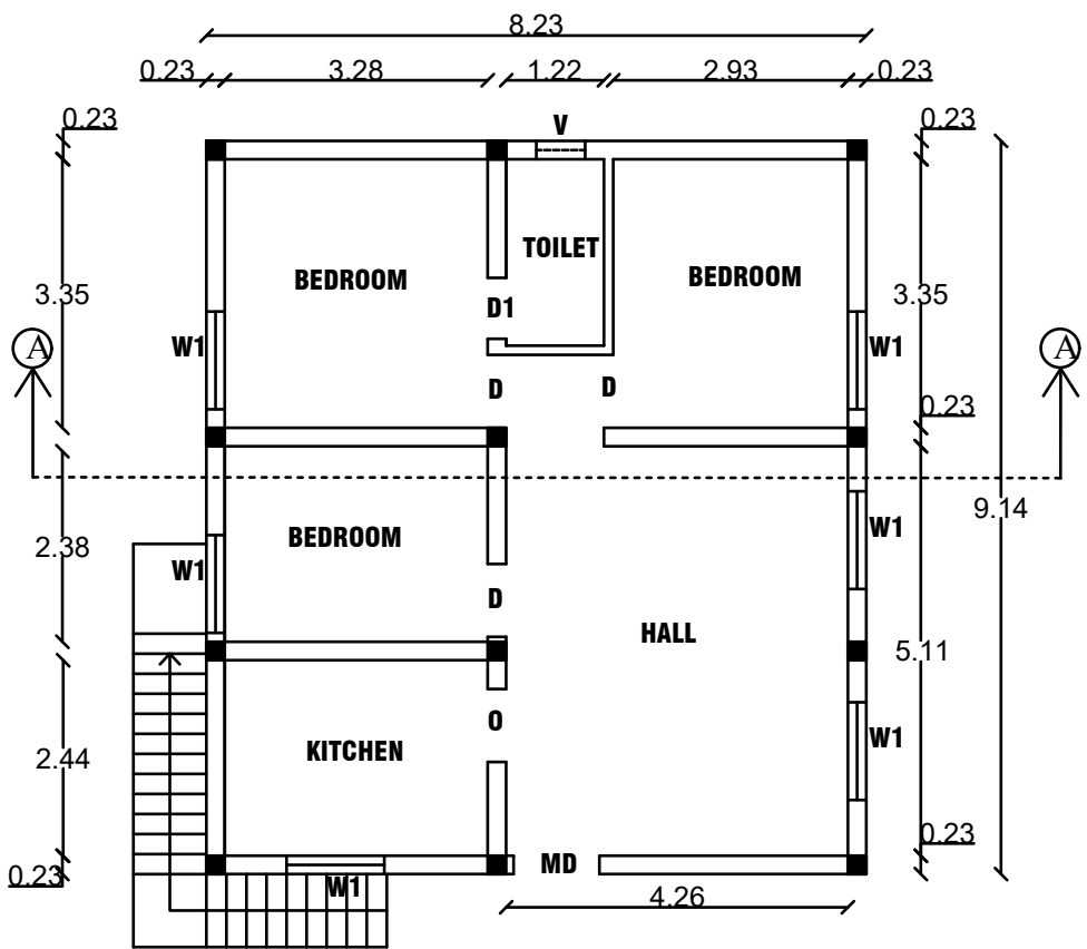
GROUND FLOOR PLAN EAST FACING PLAN
