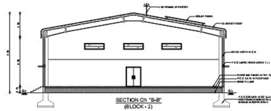
ELEVATION (BLOCK - 2)
