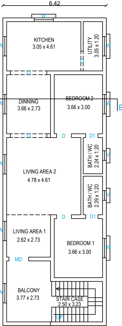
PRO.FIRST FLOOR
