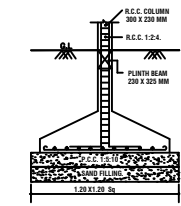
FOUNDATION DETAIL
