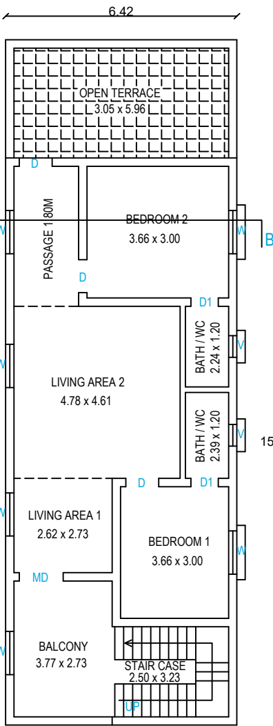
PRO.SECOND FLOOR
