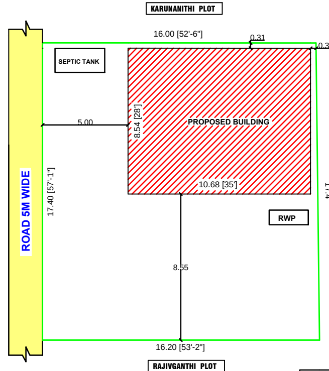
SITE PLAN
