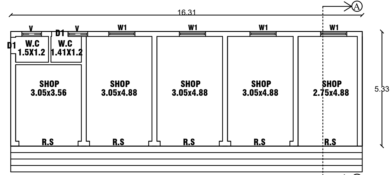
GROUND FLOOR PLAN NORTH FACING PLAN
