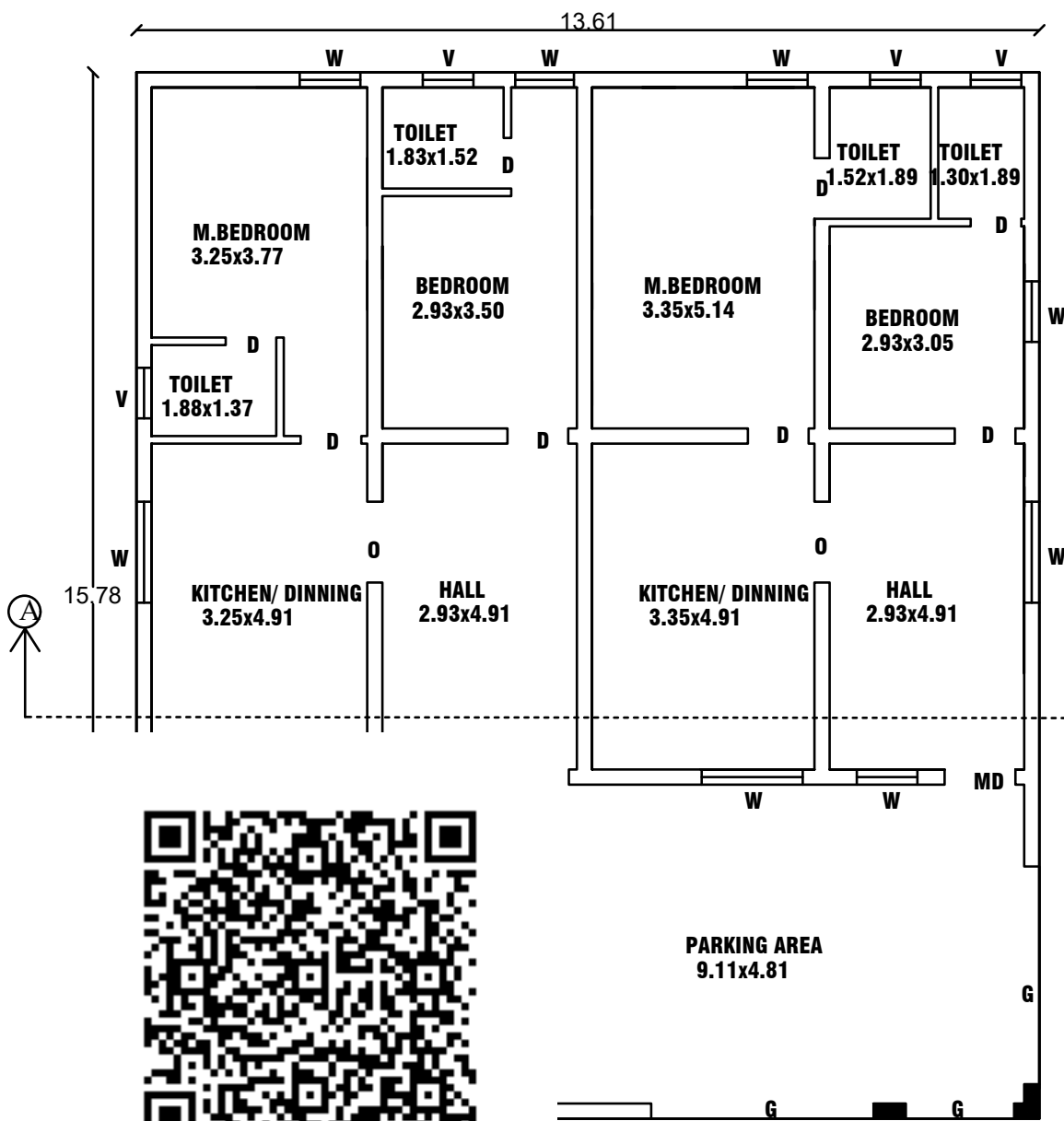
FLOOR PLAN EAST FACING PLAN
