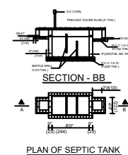
PLAN OF SEPTIC TANK
