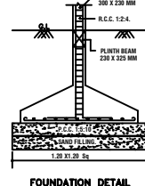
FOUNDATION DETAIL
