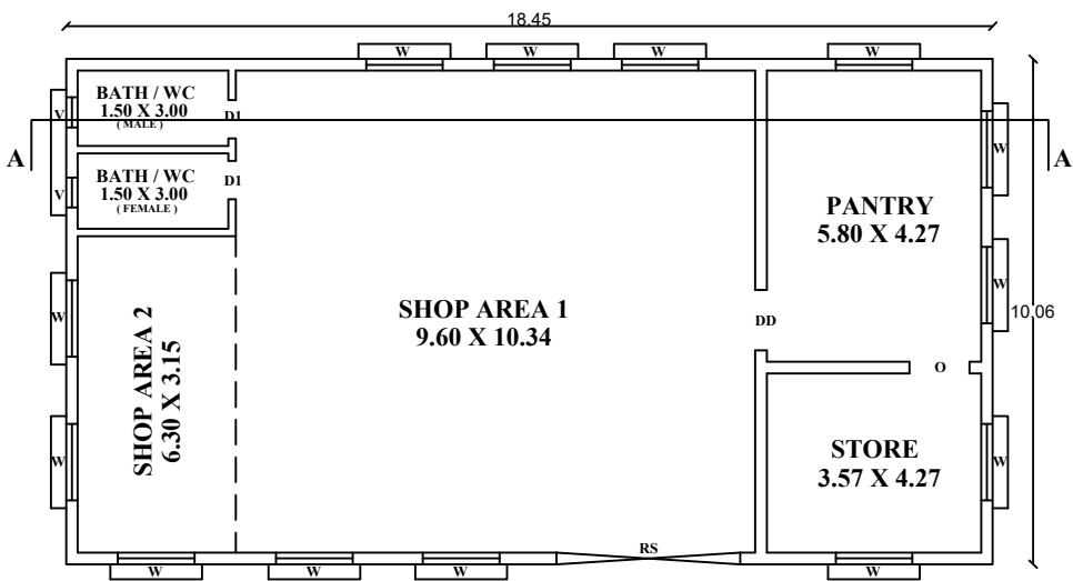
PRO. GROUND FLOOR
