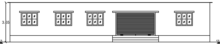
FRONT ELEVATION
