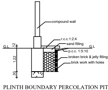
PLINTH BOUNDARY PERCOLATION PIT
