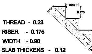
DETAIL OF STAIRCASE
