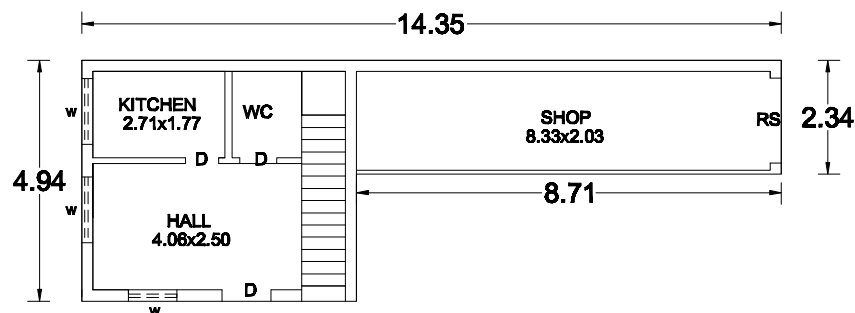
GROUND FLOOR HOUSE & SHOP PLAN EAST & NORTH FACING
