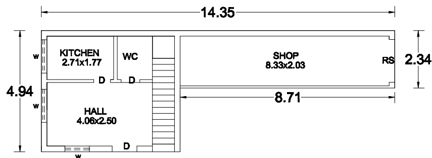
FIRST FLOOR HOUSE & SHOP PLAN EAST & NORTH FACING
