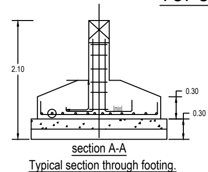
Typical section through footing.
