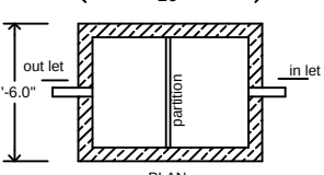
DETAILS OF SEPTIC TANK
