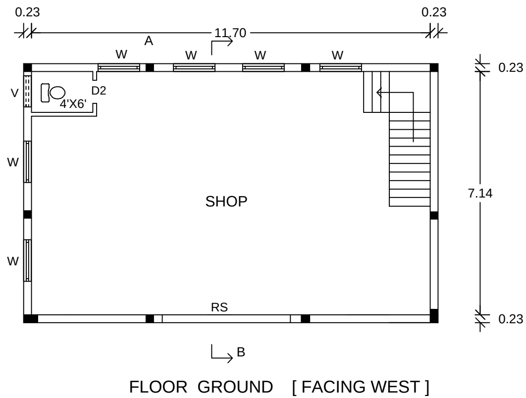
FLOOR GROUND [FACING WEST]
