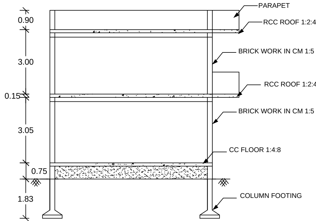
SECTION AB
