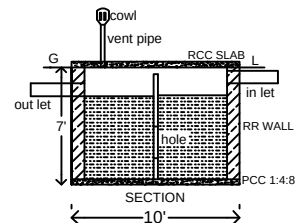
RAIN WATER HARVEST PIT
