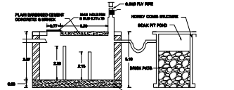
SECTION X-X DETAIL OF SEPTIC TANK, [ SCALE 1:200 ]
