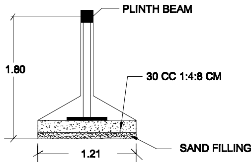
COLUMN DETAILS
