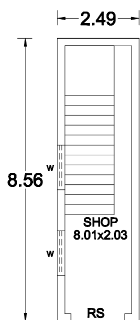
GROUND FLOOR SHOP NORTH FACING
