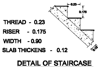
DETAIL OF STAIRCASE
