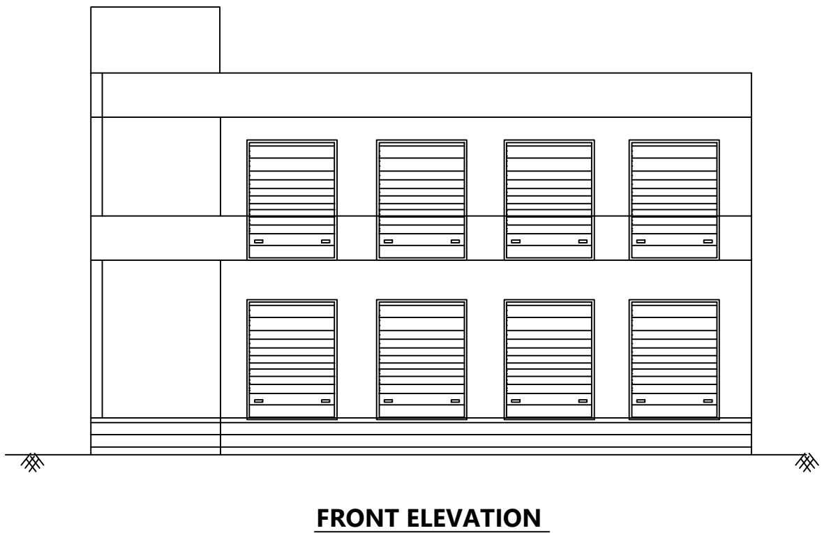
FRONT ELEVATION
