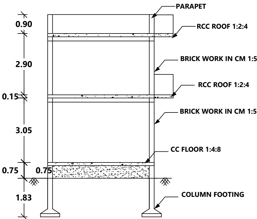
SECTION AB
