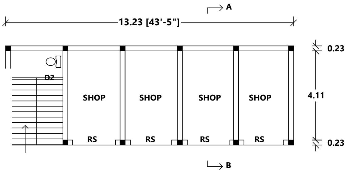
FLOOR GROUND
