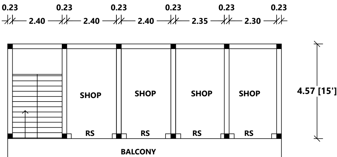
FLOOR 01
