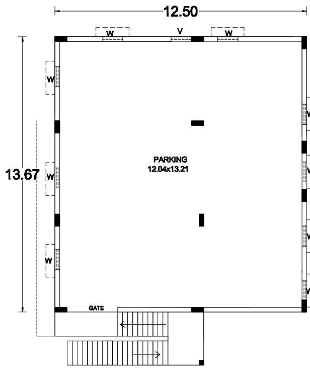
STILT FLOOR PLAN NORTH FACE
