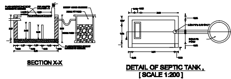
PERCOLATION PIT SECTION OF RAIN WATER
