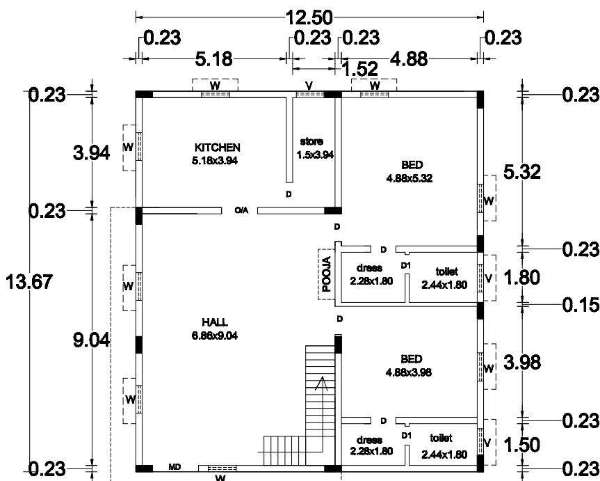
SECOND FLOOR PLAN NORTH FACE
