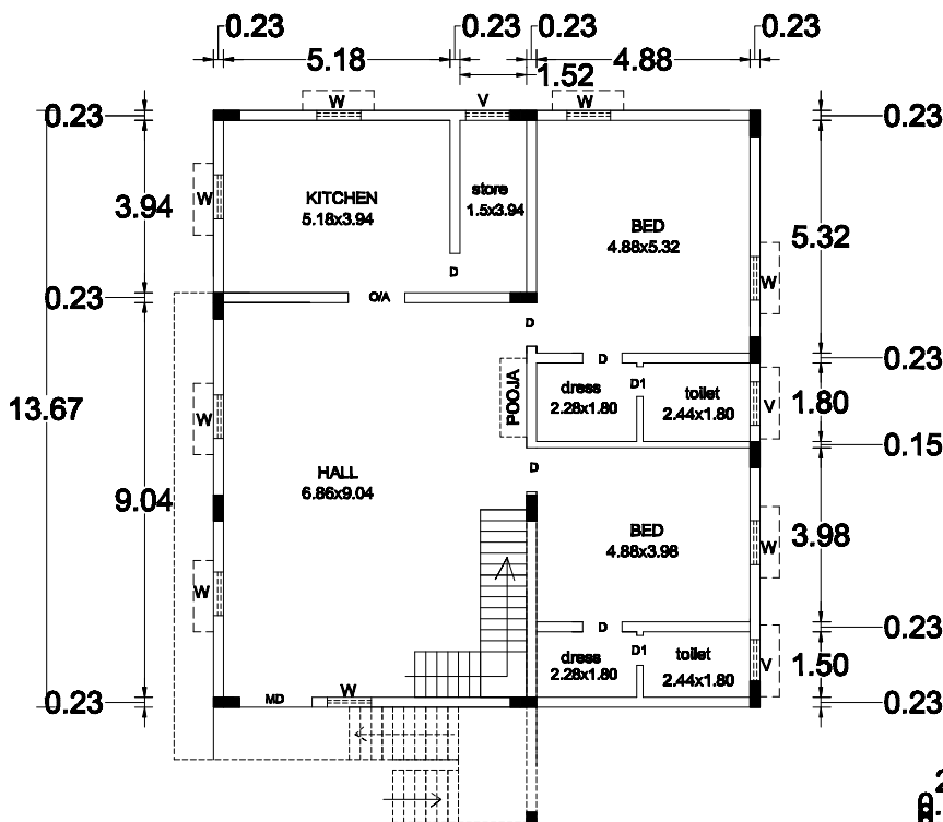
FIRST FLOOR PLAN NORTH FACE
