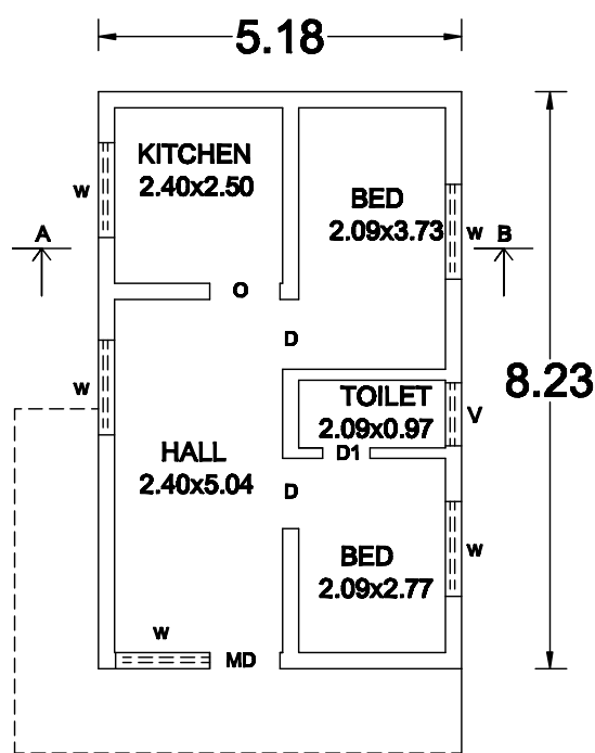
GROUND FLOOR PLAN NORTH FACE
