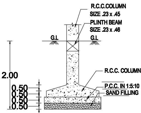
FOUNDATION DETAIL (DETAIL - B)
