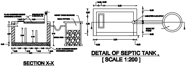
SECTION X-X
