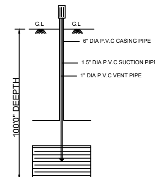
BORE WELL
