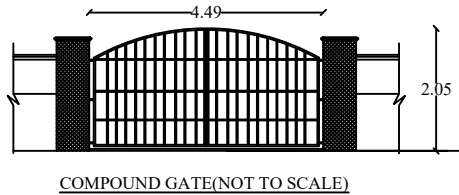
COMPOUND GATE(NOT TO SCALE)
