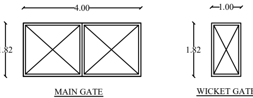
WICKET GATE
