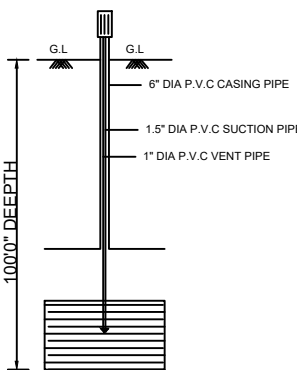
BORE WELL
