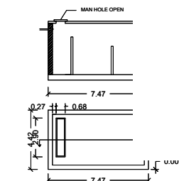
DETAIL OF SEPTIC TANK
