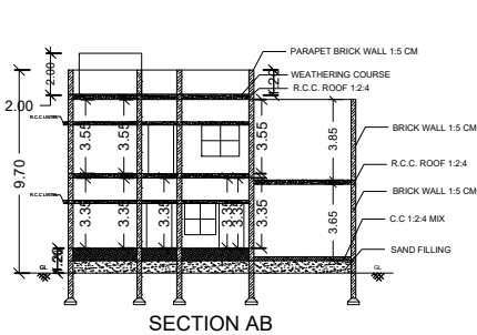
SECTION AB
