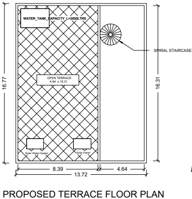
PROPOSED TERRACE FLOOR PLAN
