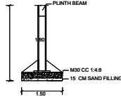
COLUMN DETAILS
