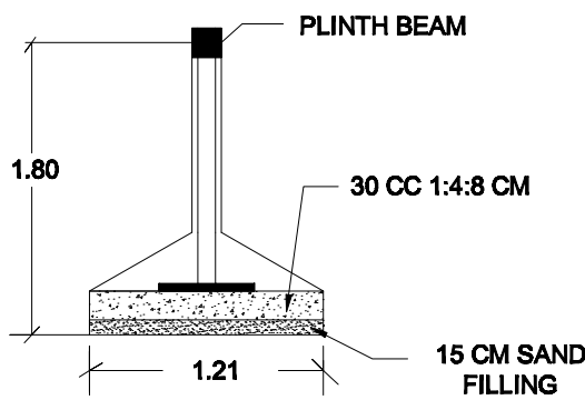
COLUMN DETAILS
