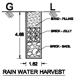
RAIN WATER HARVEST
