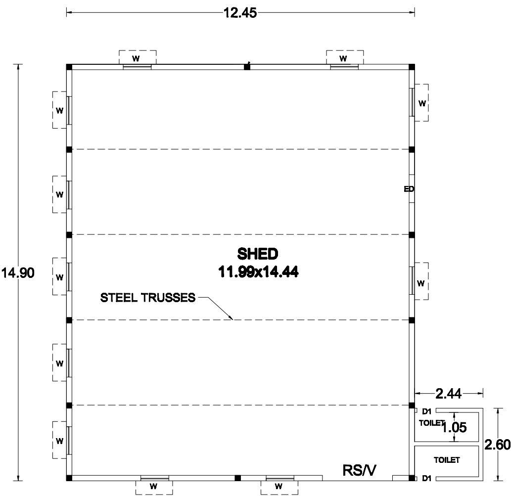
PI AN OF COMMERCIAL SHED
