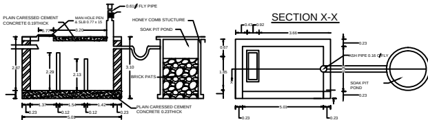
DETAIL OF SEPTIC TANK [ SCALE 1:200 ]
