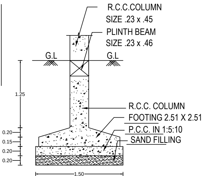
FOUNDATION DETAIL (DETAIL - B)
