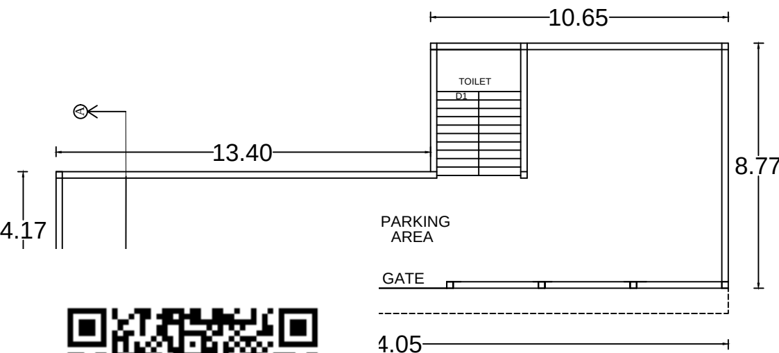
LOOR PLAN
