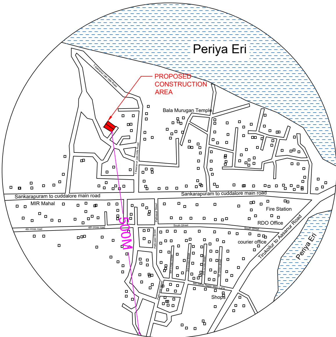
TOPO PLAN SCALE : 1:1000
