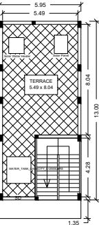
TERRACE FLOOR PLAN
