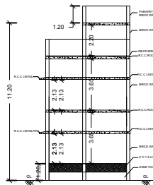
SECTION AB
