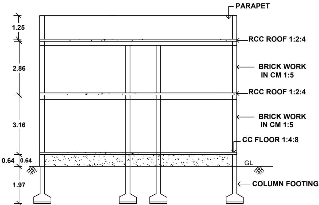
SECTION AB
