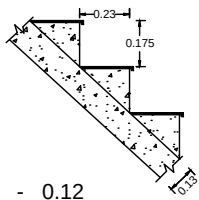
DETAIL OF STAIRCASE
