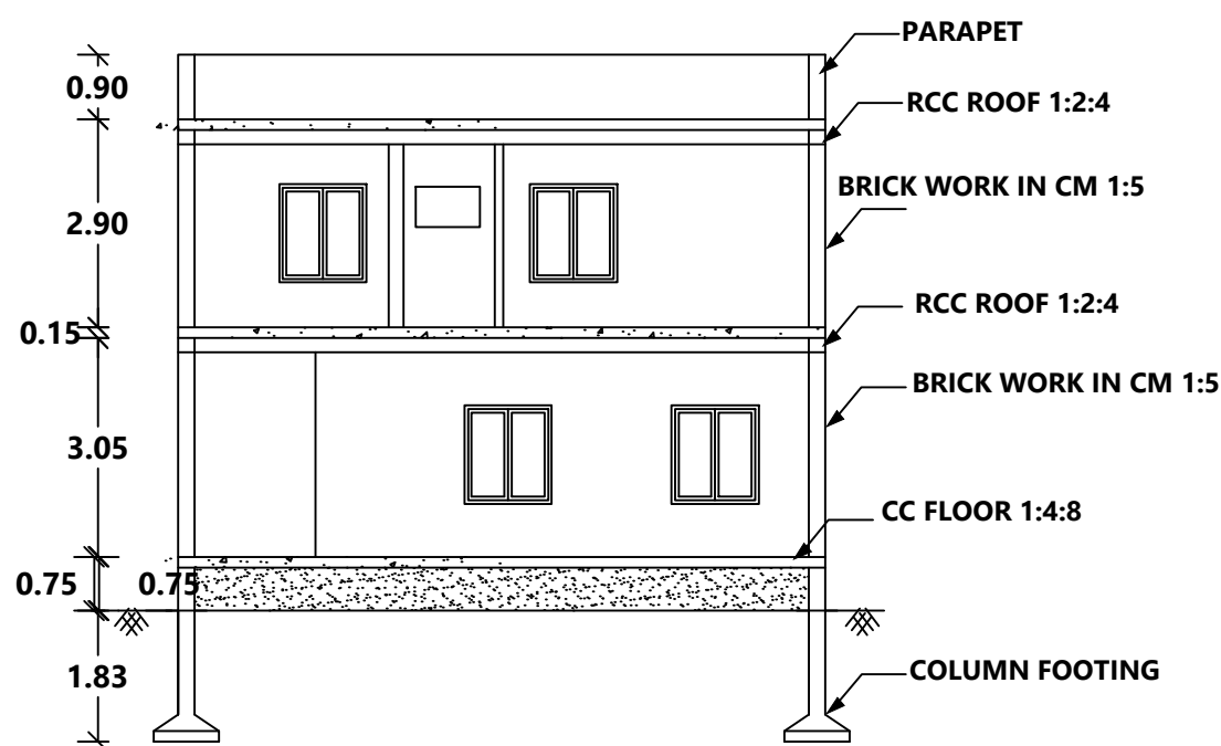
SECTION AB
