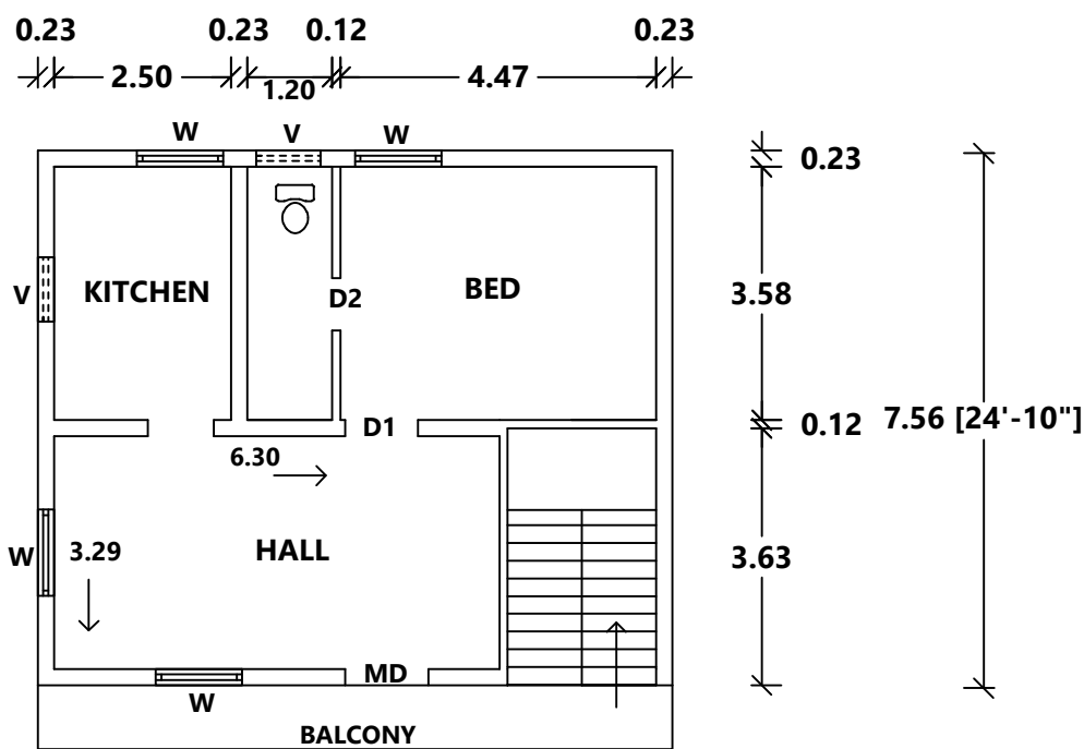
FLOOR 01
