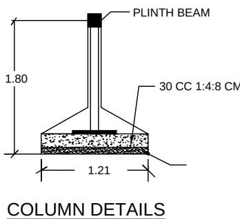
COLUMN DETAILS
