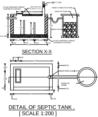
DETAIL OF SEPTIC TANK. [SCALE 1:200]
