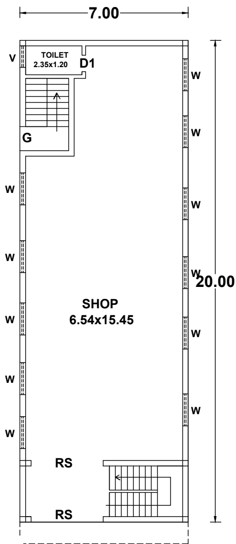
GROUND FLOOR PLAN- commercial
