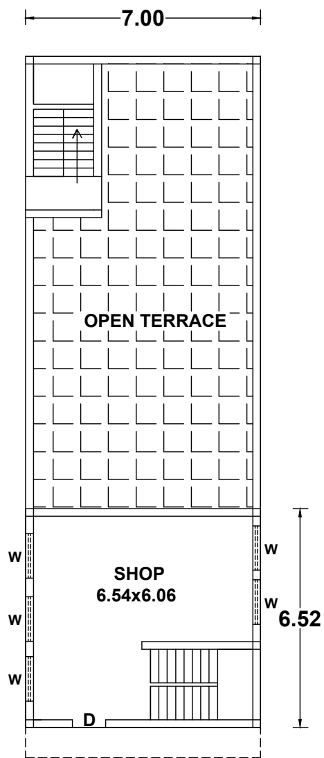
FIRST FLOOR PLAN- commercial
