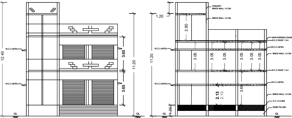
SECTION AB
