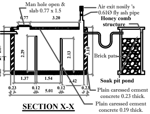
SECTION X-X
