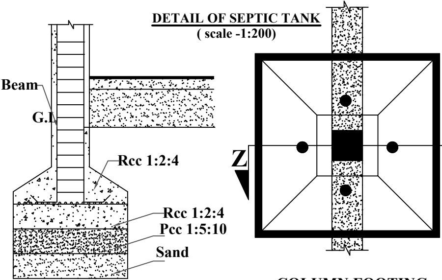
SECTION Z-Z SCALE 1:200
