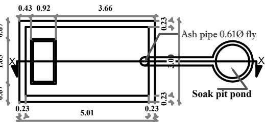
DETAIL OF SEPTIC TANK (scale -1:200)
