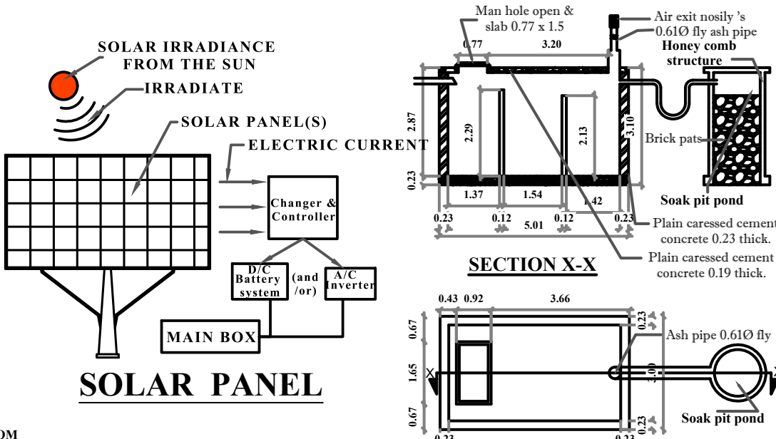
DETAIL OF SEPTIC TANK (scale -1:200)
