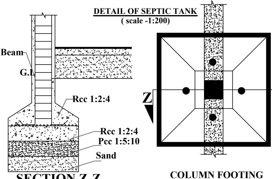
SECTION Z-Z SCALE 1:200
