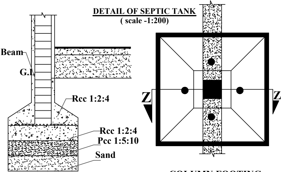
SECTION Z-Z SCALE 1:200
