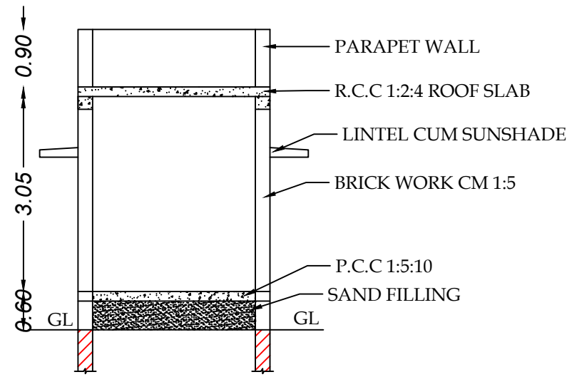
SECTION AB
