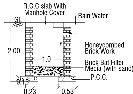
DETAILS OF RAIN WATER COLLECTION PIT SCALE:- 1"=4'0"
