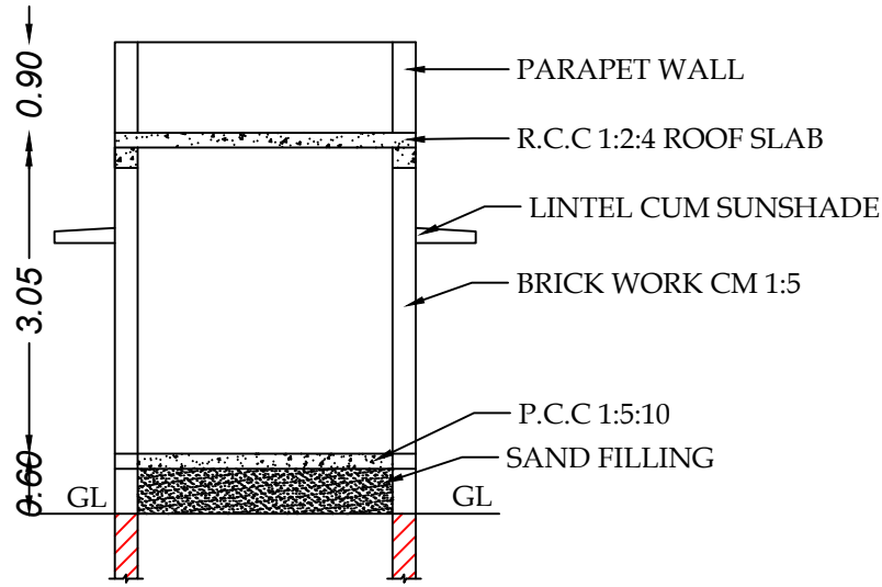
SECTION AB
