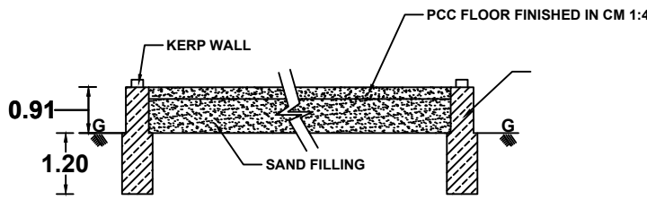
SECTION ON DRYING YARD
