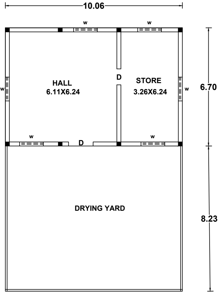
PLAN OF GODOWN
