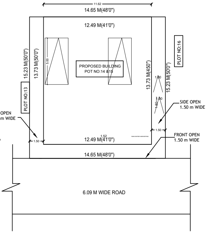
SITE PLAN
