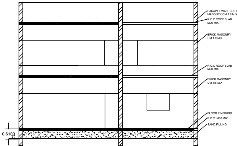
SECTION ON-AA
