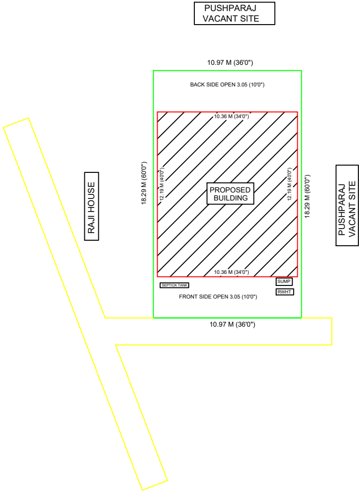
SITE PLAN TO SCALE
