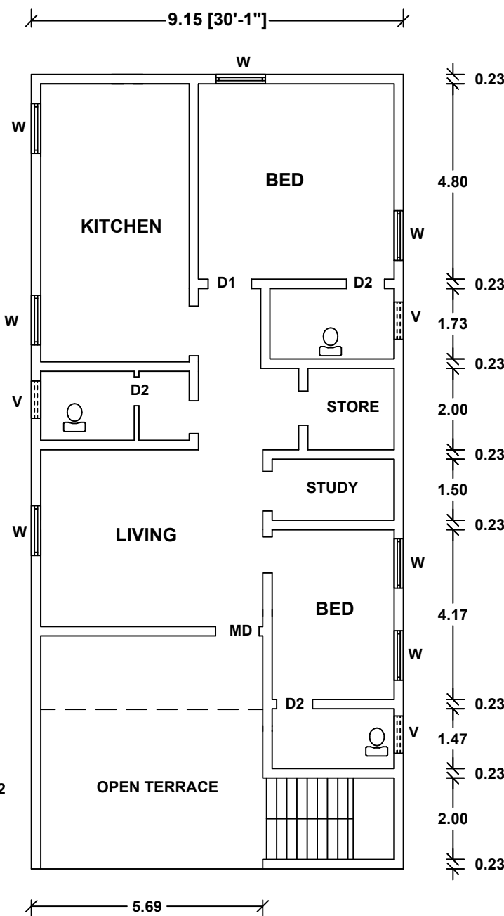
FLOOR 01
