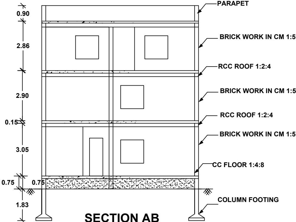
SECTION AB
