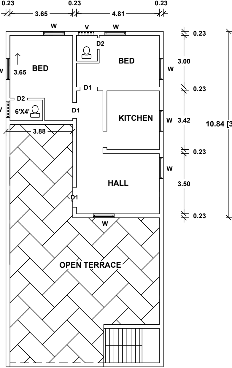
FLOOR 02
