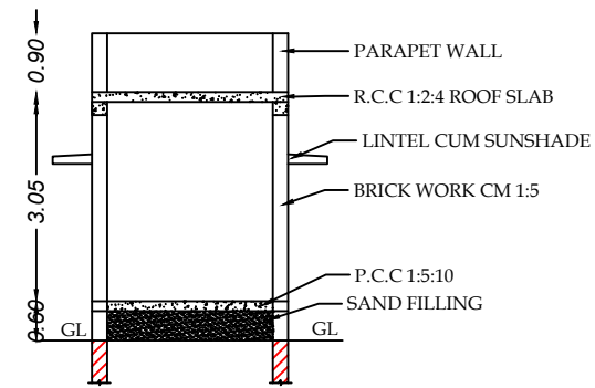
SECTION AB
