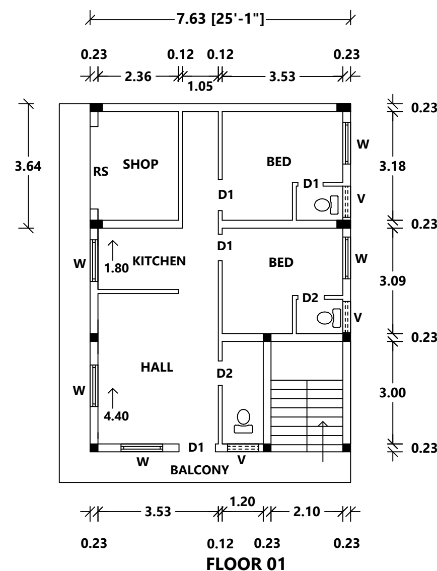
FLOOR 01
