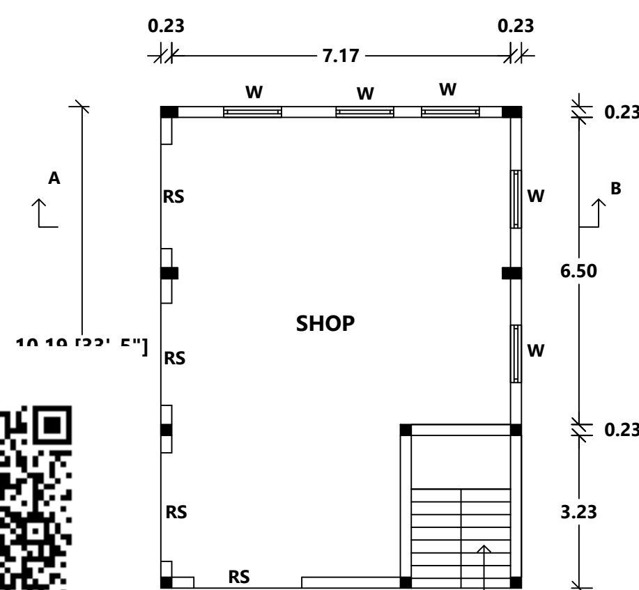
FLOOR GROUND
