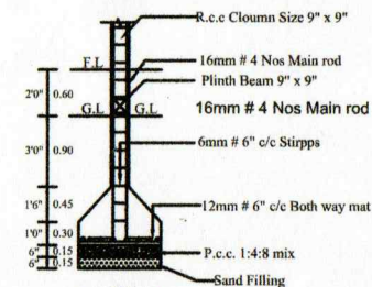
COLUMN DETIAL
