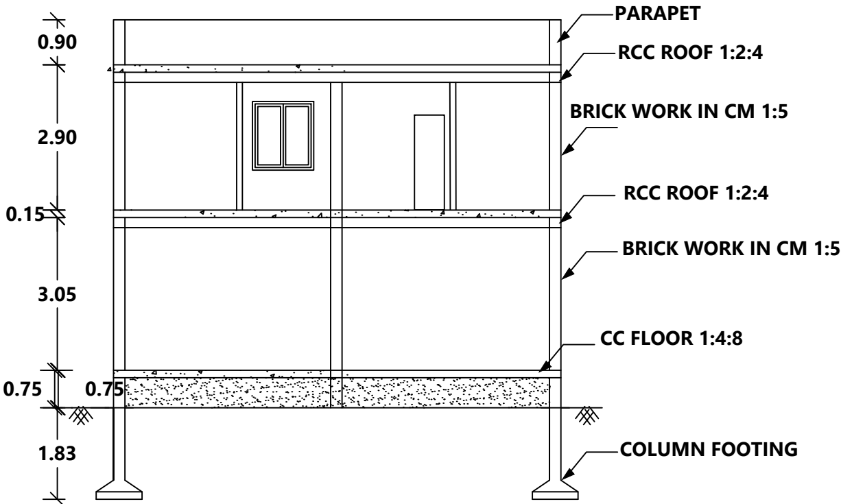
SECTION AB
