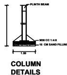
COLUMN DETAILS
